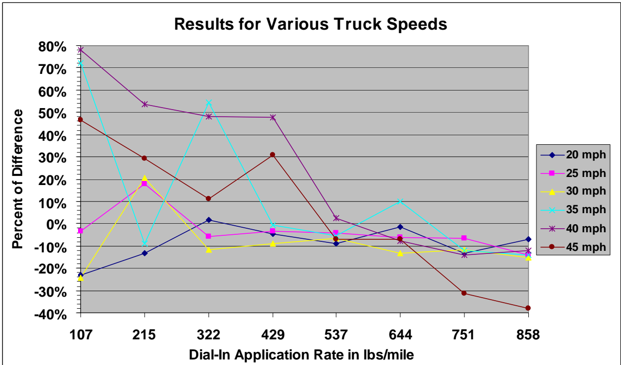
Figure K-5. Percent of Difference between Actual Solid Discharge Rate and Dial-In Solid Application Rate as a Function of Dial-In Solid Application Rate
