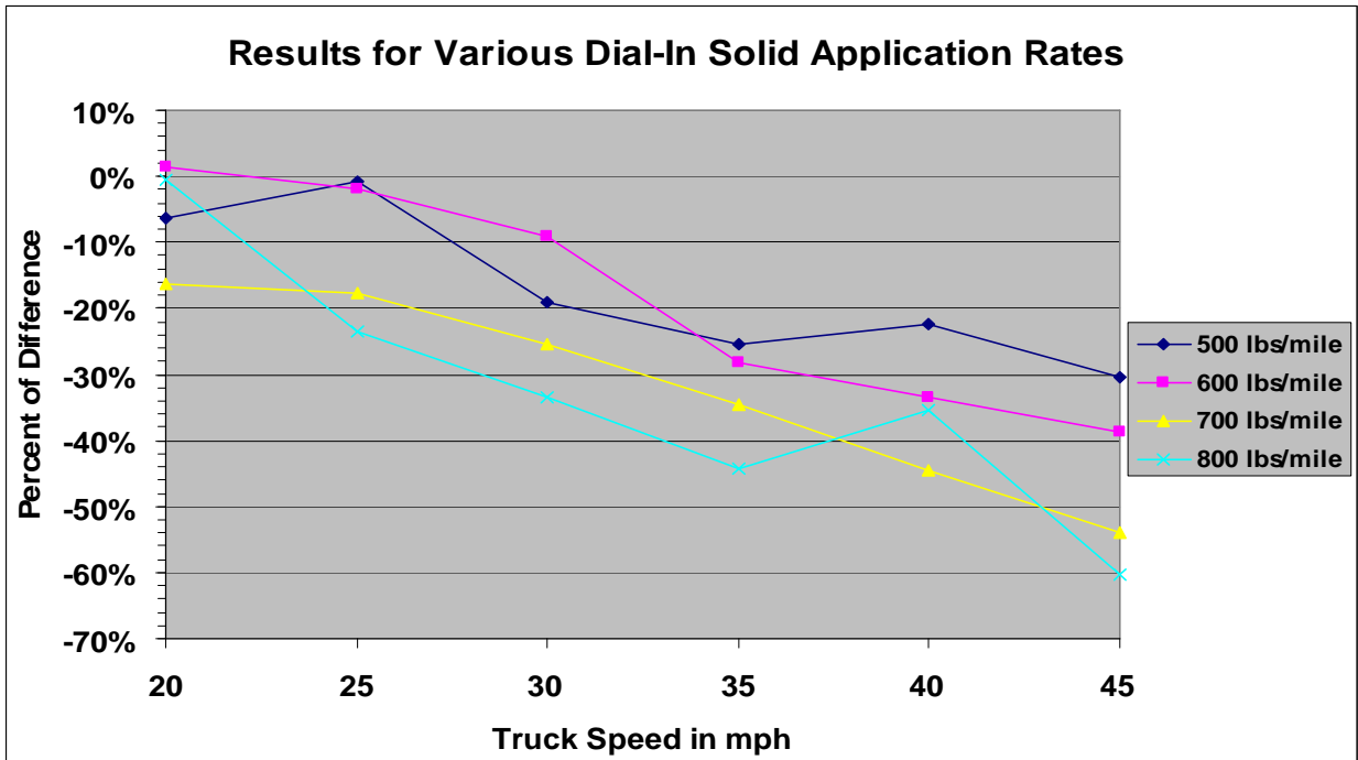
Figure F-4. Percent of Difference between Actual Solid Discharge Rate and Dial-In Solid Application Rate as a Function of Truck Speed
