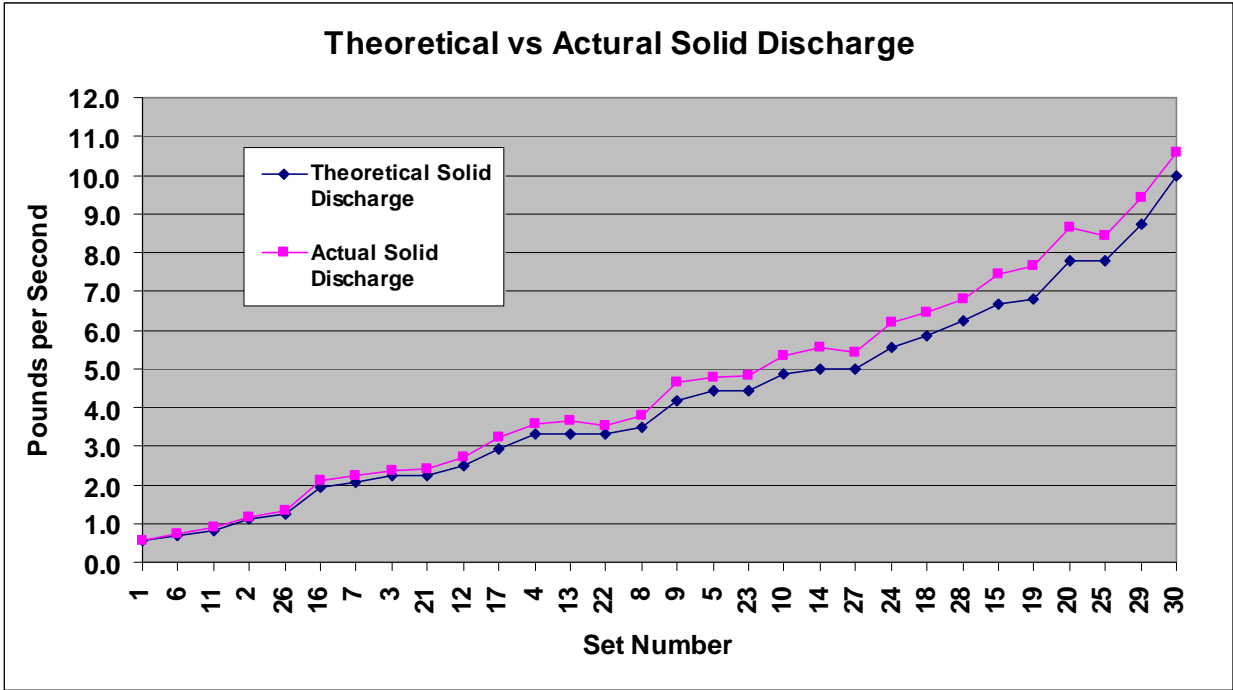
Figure J-1. Theoretical Vs Actual Solid Discharge Rate
