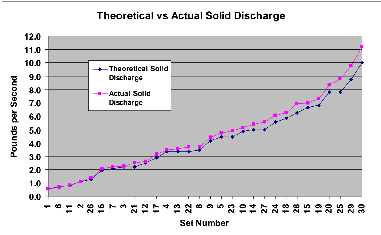
Figure H-6. Theoretical vs Actual Solid Discharge Rate
